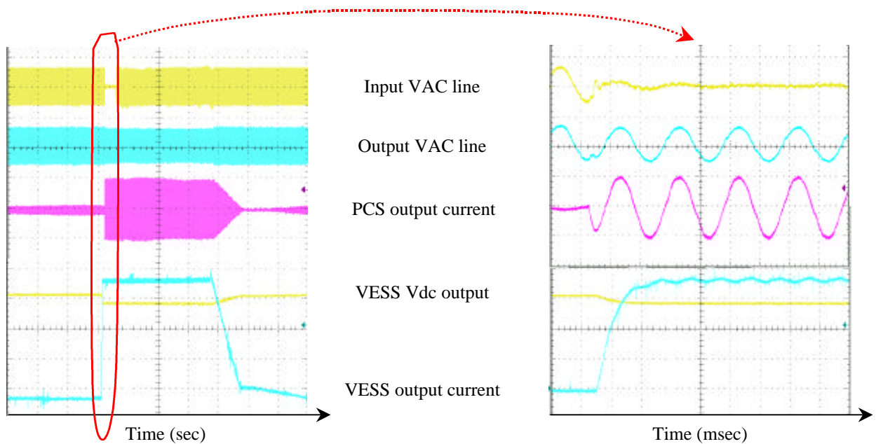
Fig 5.: Short-time response
